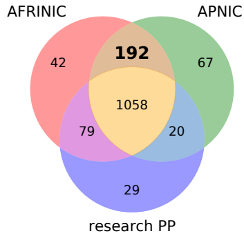
Figure 9: Set diagram showing the overlap of RP IP addresses seen across three PPs on March 30, 2020 (proportions not to scale).
